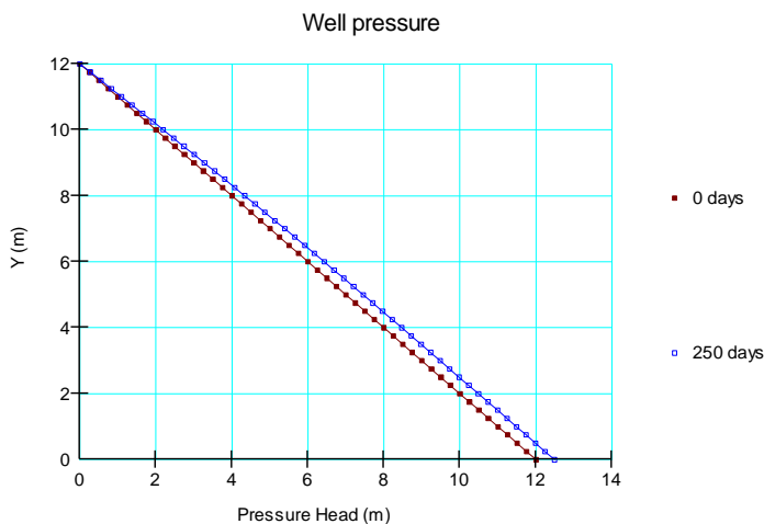
Figure 12 Excess pressure head distribution in the well
