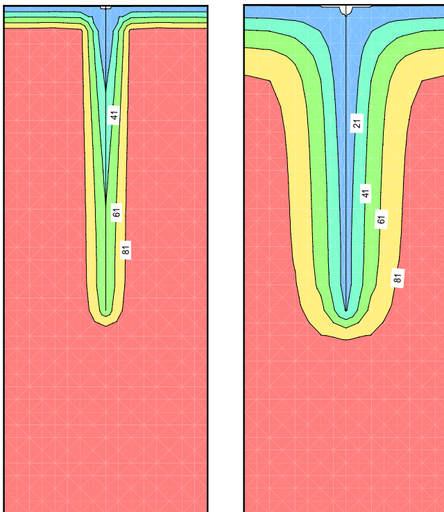
Figure 6 Pore-pressure distributions on Day 1 and Day 6
