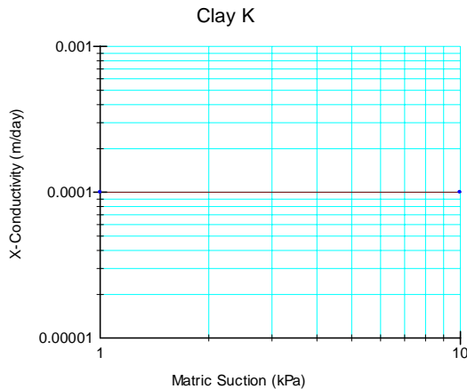
Figure 4 Hydraulic conductivity function for the clay
