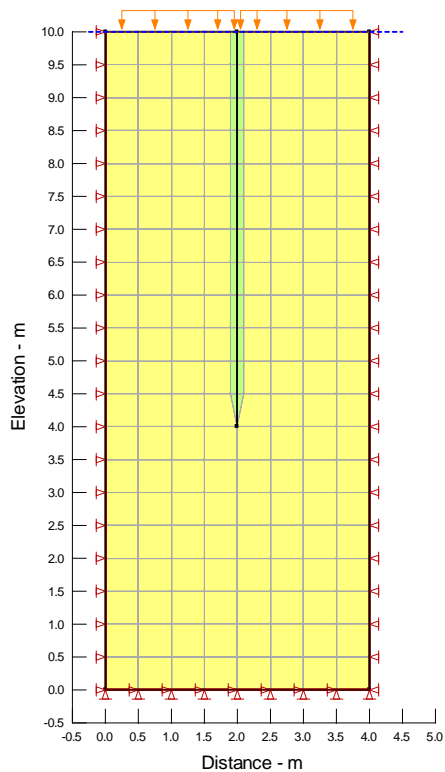
Figure 1 Configuration of wick drain cell
