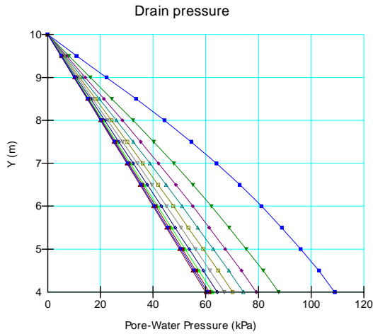
Figure 5 Pressure distributions in the drain
