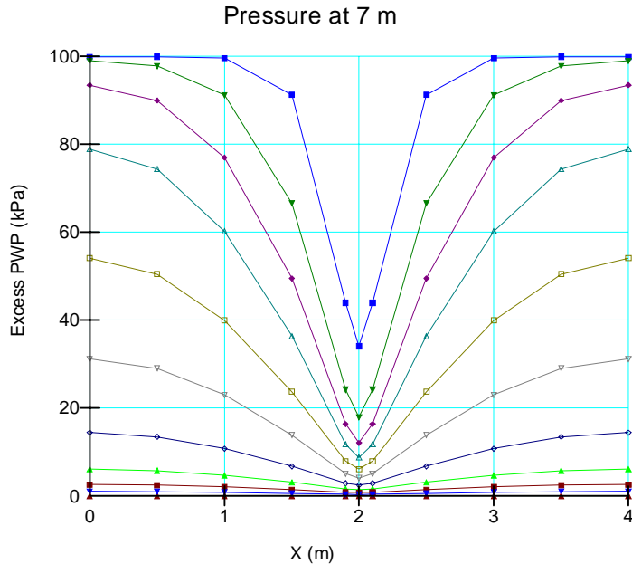
Figure 7 Pressure changes at El. 7 m
