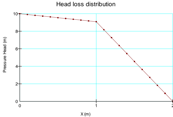
Figure 9 Head loss distribution in a layered system
