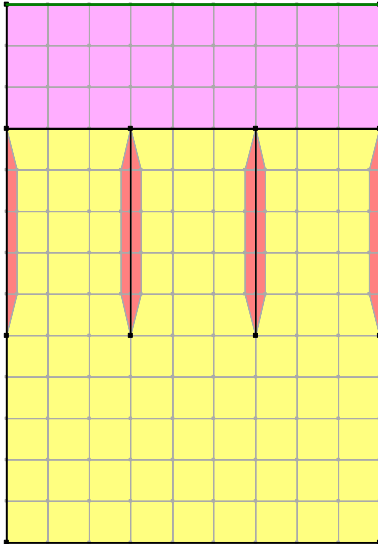
Figure 10 Layout with granular layer above the drains
