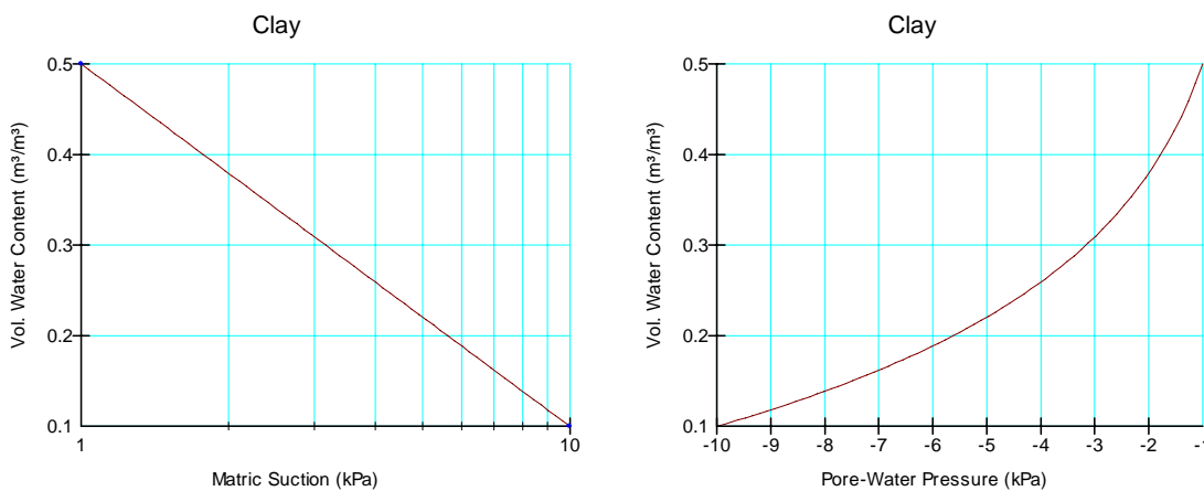
Figure 3 Volumetric Water Content function
