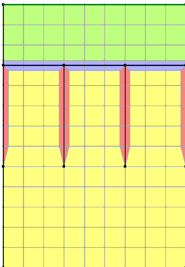
Figure 11 Layout with horizontal interface layer for lateral drainage
