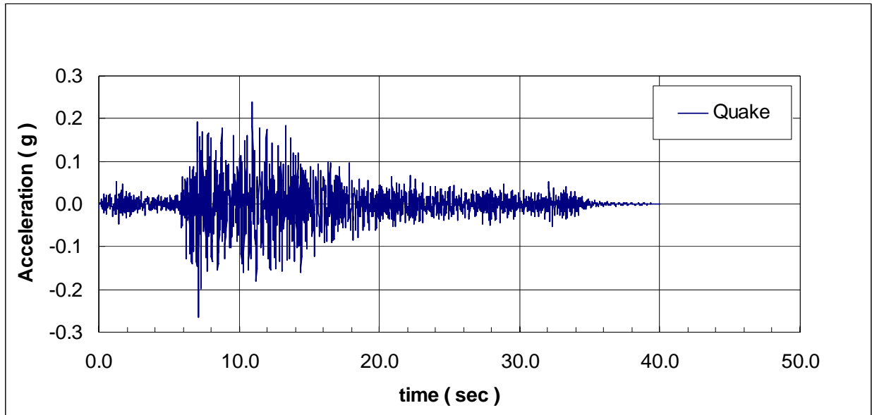
Figure 34 Saguenay ground surface acceleration
