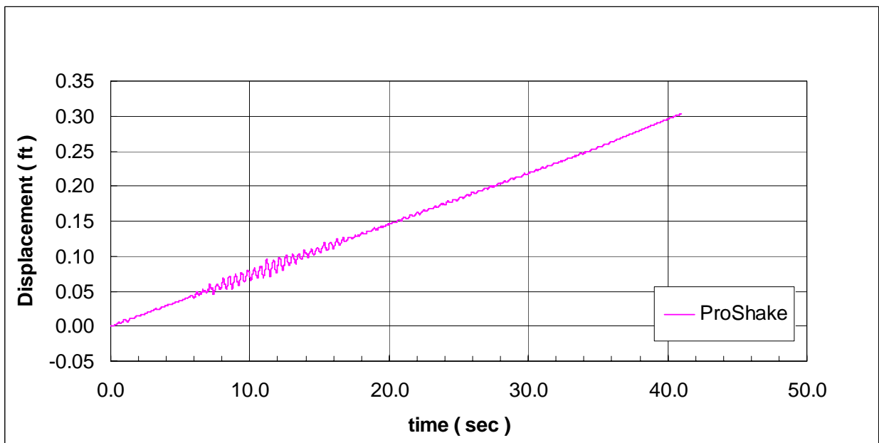
Figure 37 Saguenay ground surface displacements
