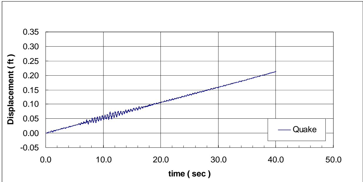
Figure 38 Saguenay ground surface displacements
