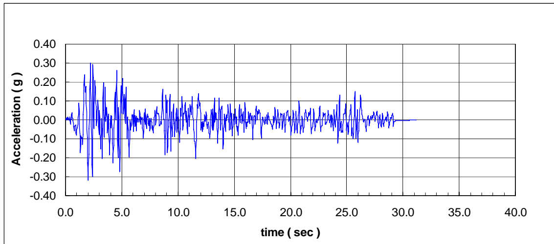
Figure 5 The El Centro Earthquake
