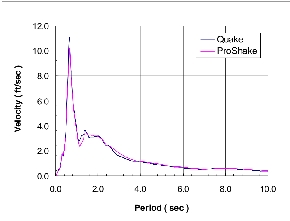
Figure 11 Treasure Island surface spectral velocities
