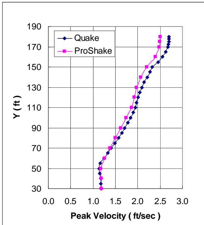
Figure 27 El Centro peak velocity profile
