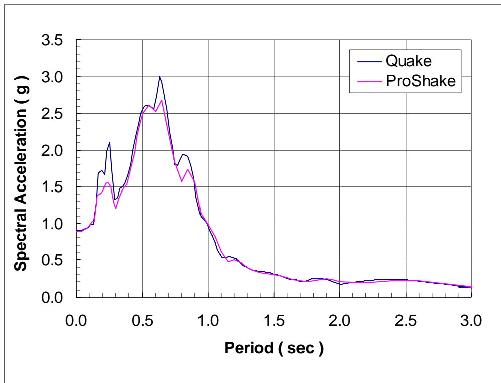
Figure 23 El Centro spectral ground surface accelerations
