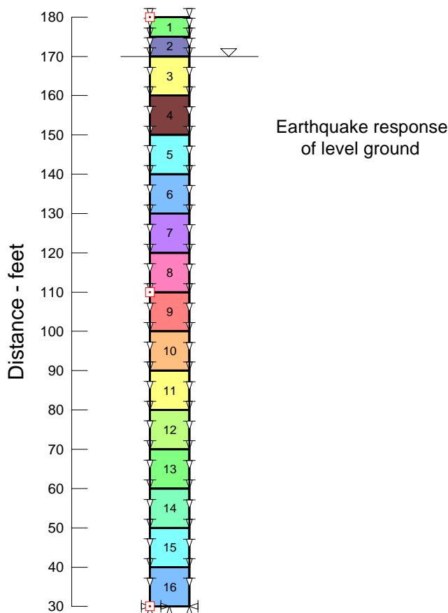
Figure 1 The SHAKE soil profile defined in QUAKE/W
