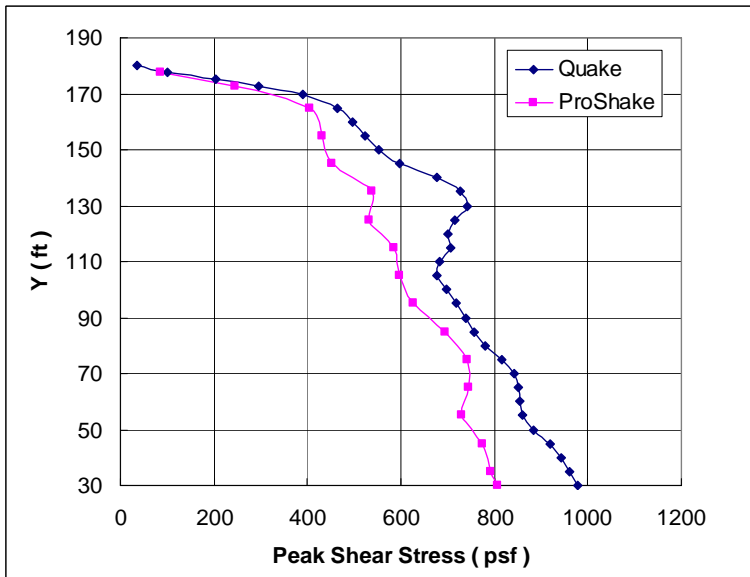
Figure 45 Saguenay peak shear stress profile
