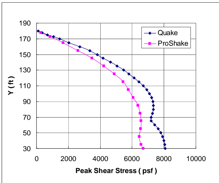
Figure 29 El Centro peak shear stress profile
