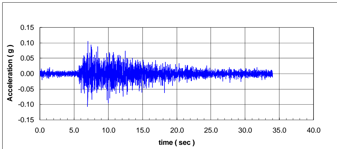
Figure 6 The Saguenay Earthquake
