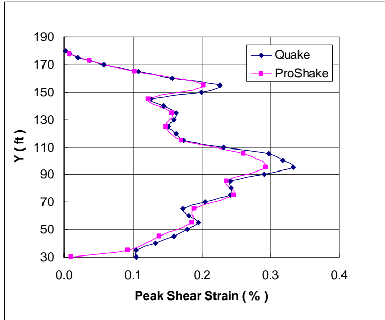
Figure 30 El Centro peak shear strain profile
