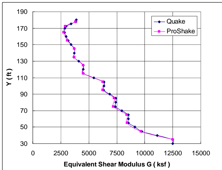
Figure 47 Saguenay equivalent shear modulus profile
