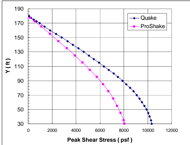
Figure 16 Treasure Island peak shear stress profile
