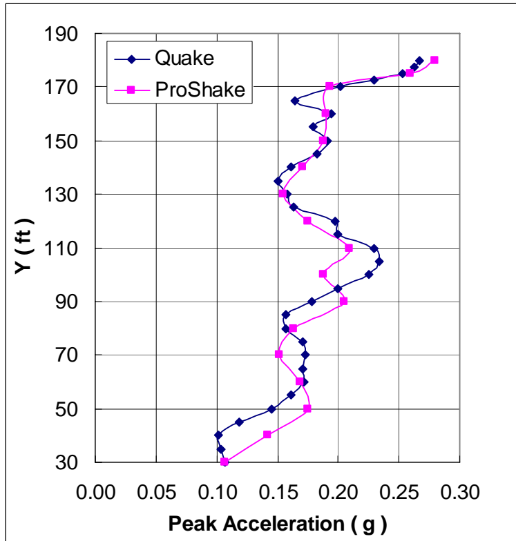
Figure 42 Saguenay peak acceleration profile
