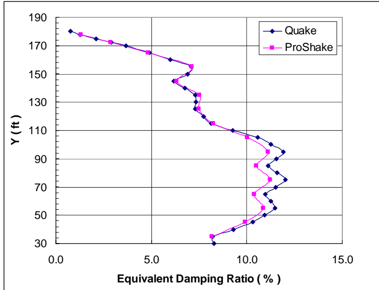
Figure 19 Treasure Island equivalent damping ratio profile
