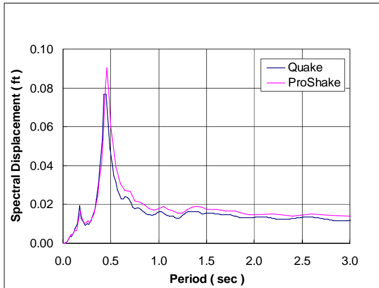
Figure 41 Saguenay spectral ground surface displacements
