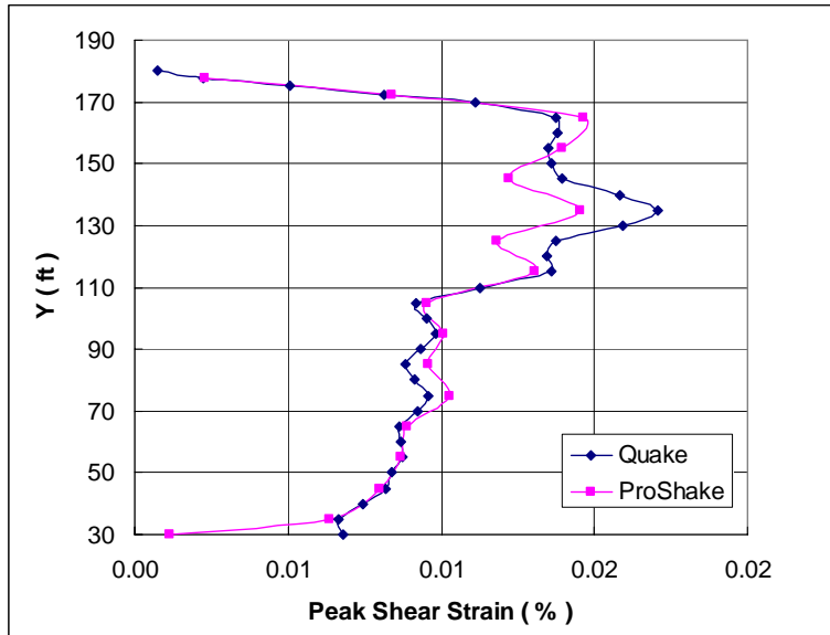
Figure 46 Saguenay peak shear strain profile
