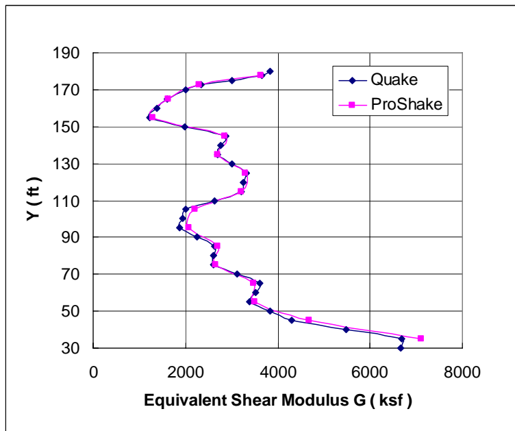
Figure 31 El Centro peak shear modulus profile
