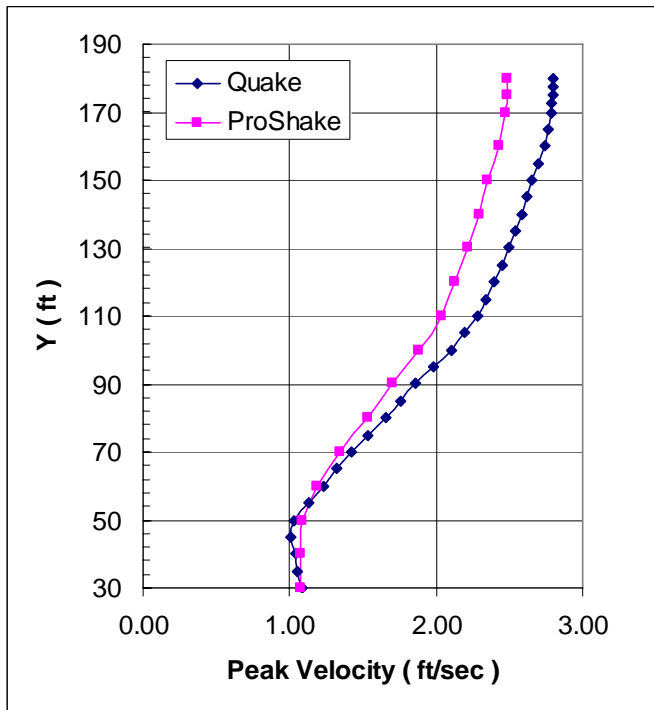
Figure 14 Treasure Island peak velocity profile
