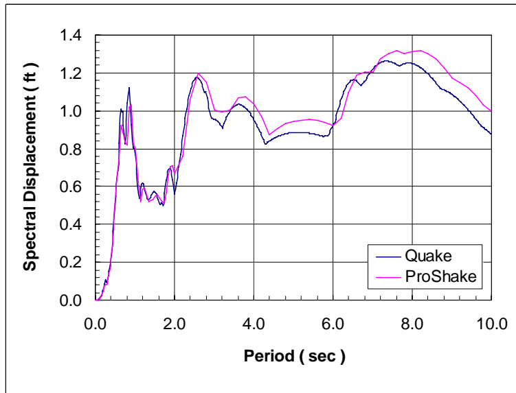
Figure 25 El Centro spectral ground surface displacement
