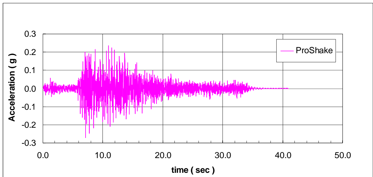
Figure 33 Saguenay ground surface acceleration
