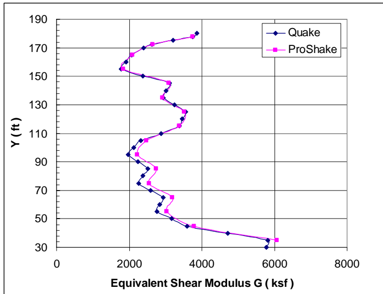
Figure 18 Treasure Island equivalent shear modulus profile
