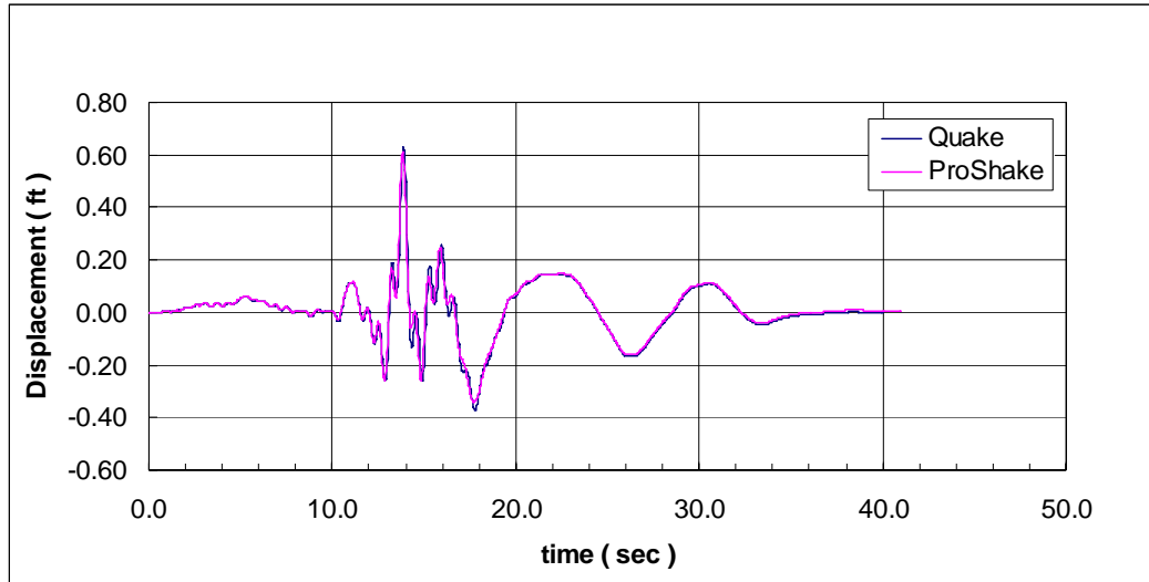
Figure 9 Treasure Island surface displacements
