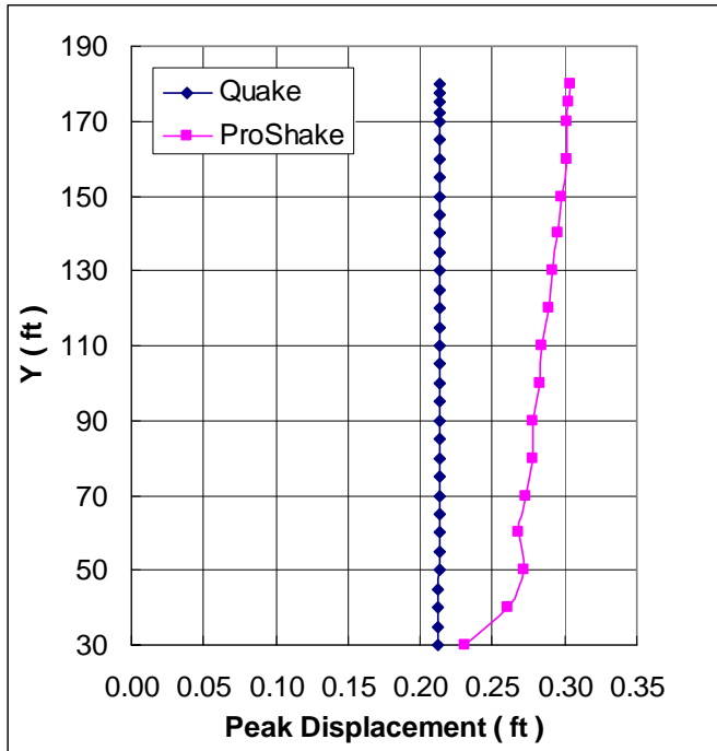
Figure 44 Saguenay peak displacement profile
