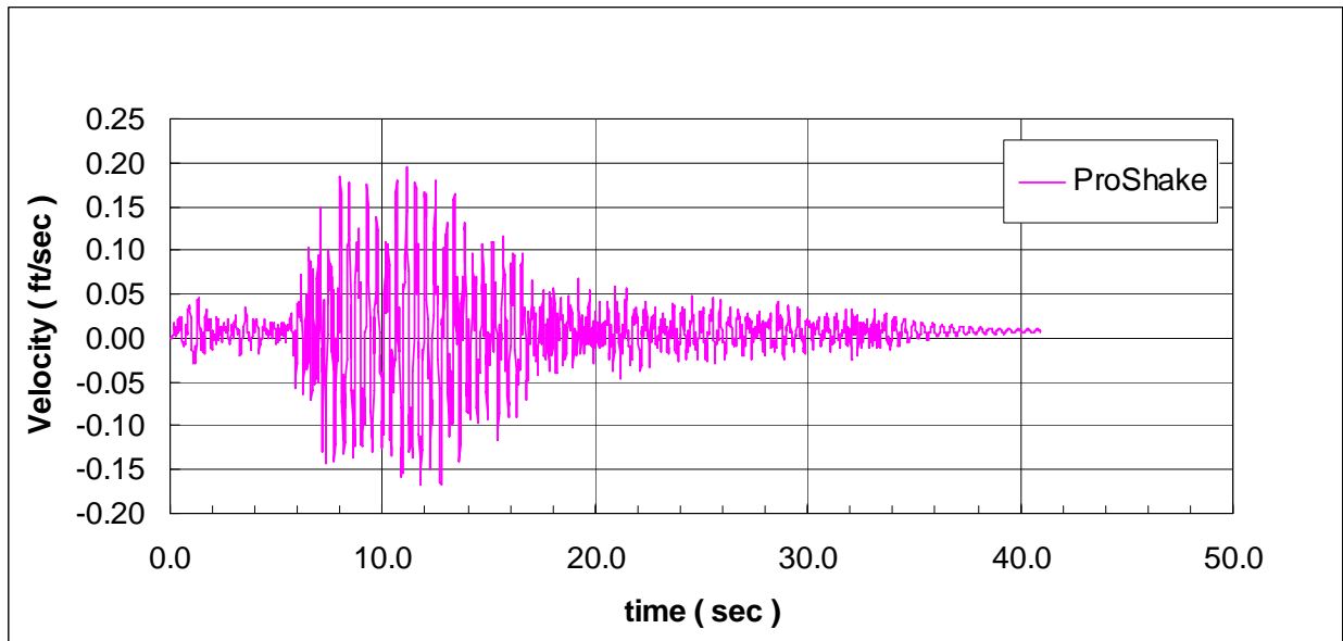
Figure 35 Saguenay ground surface velocity
