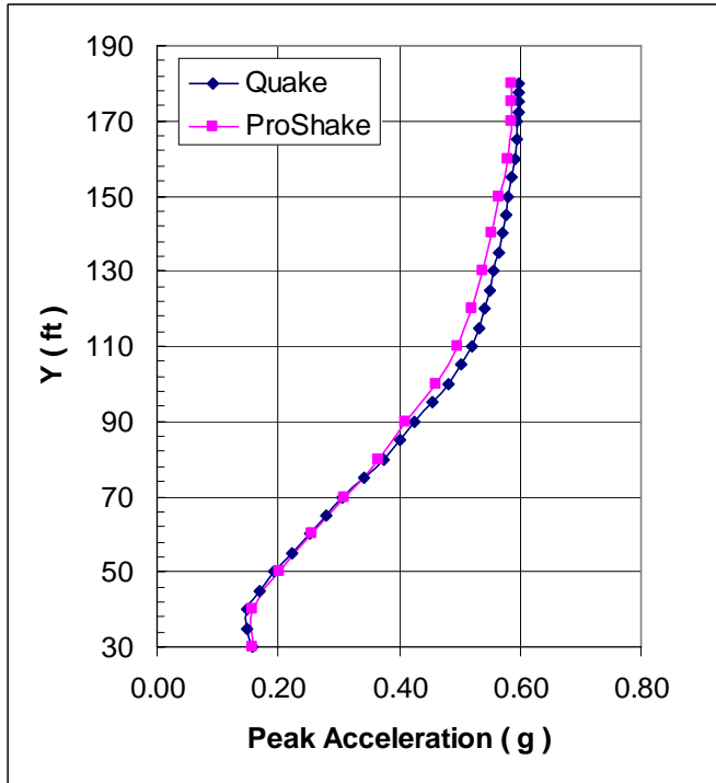
Figure 13 Treasure Island peak acceleration profile
