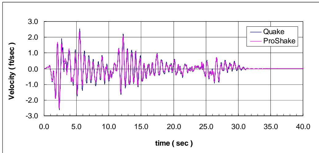
Figure 21 El Centro ground surface velocity
