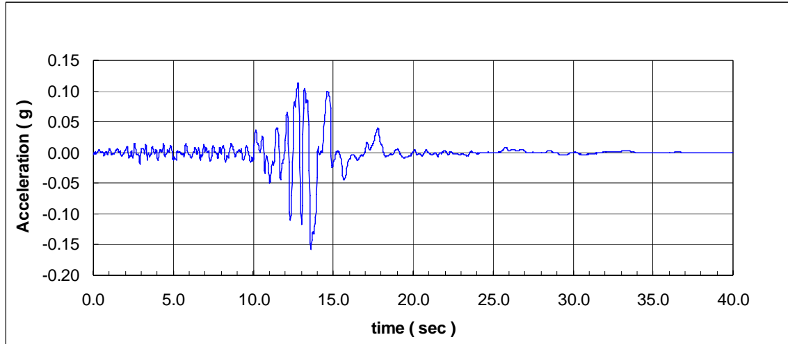
Figure 4 The Treasure Island Earthquake
