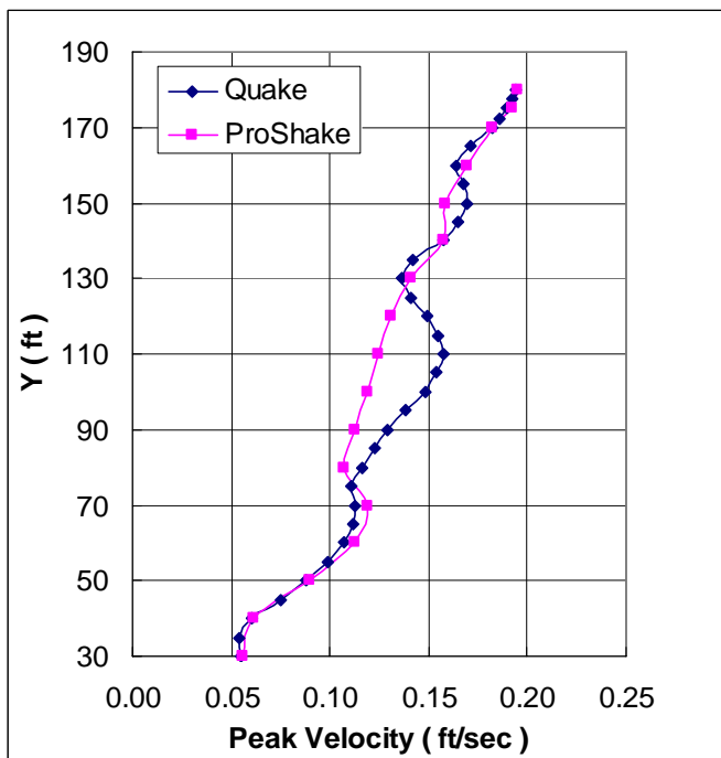
Figure 43 Saguenay peak velocity profile
