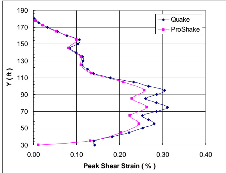
Figure 17 Treasure Island peak shear strain profile
