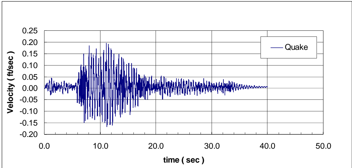
Figure 36 Saguenay ground surface velocity
