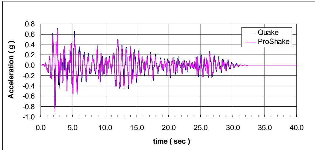
Figure 20 El Centro ground surface accelerations
