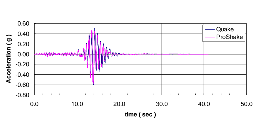
Figure 7 Treasure Island surface ground accelerations
