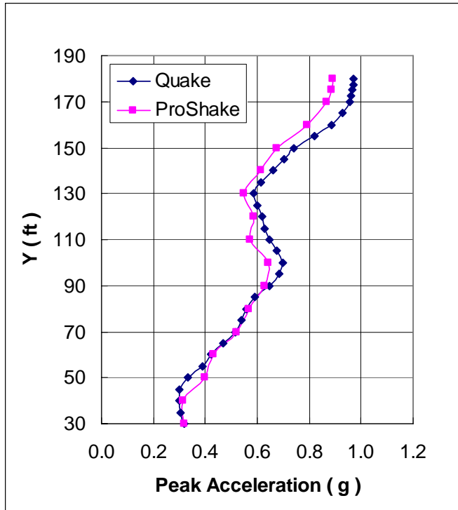
Figure 26 El Centro peak acceleration profile
