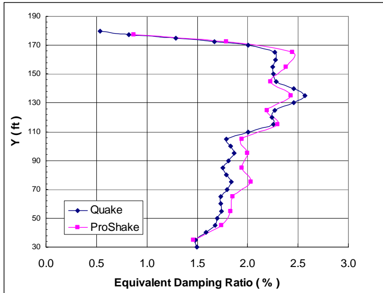
Figure 48 Saguenay equivalent damping ratio profile
