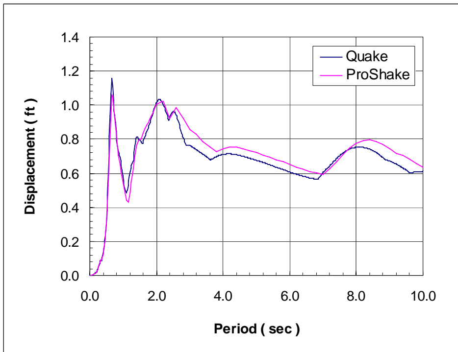
Figure 12 Treasure Island surface spectral displacements
