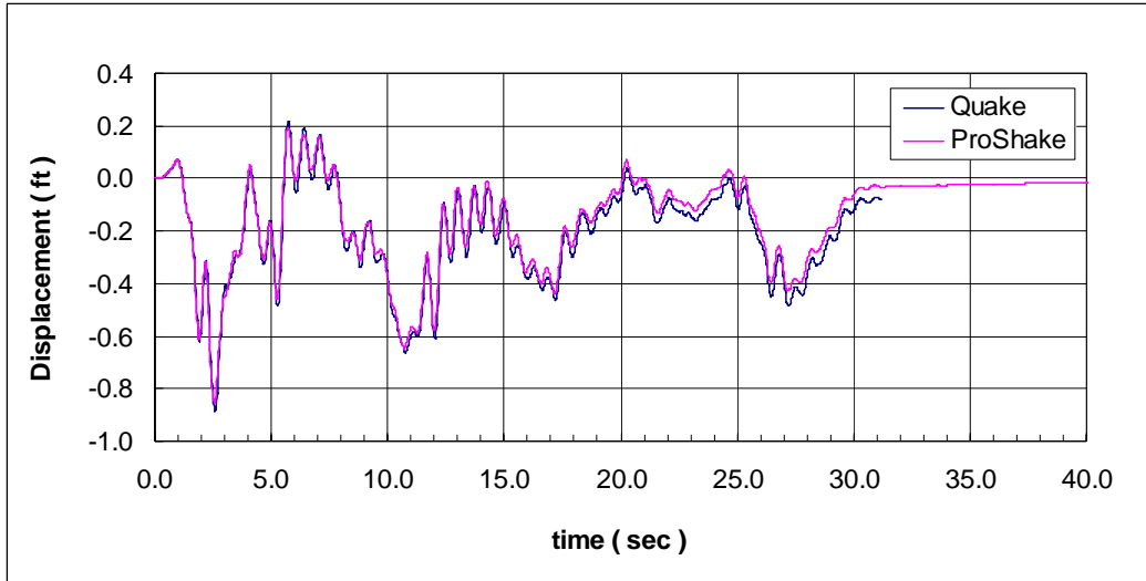
Figure 22 El Centro ground surface displacements
