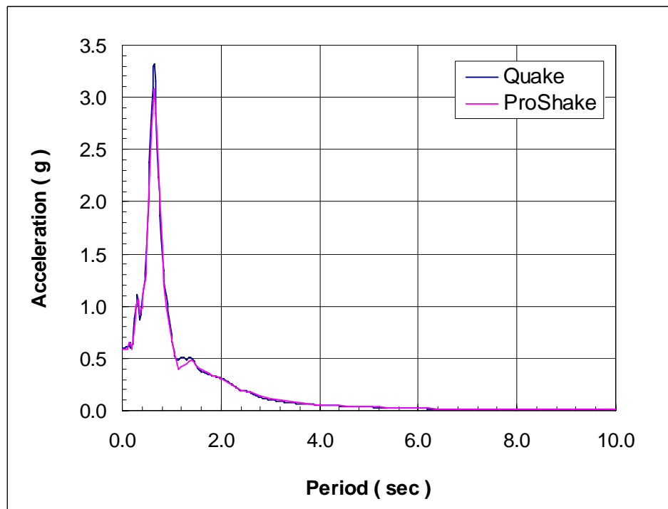
Figure 10 Treasure Island surface spectral accelerations
