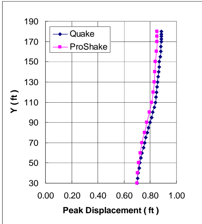
Figure 28 El Centro peak displacement profile
