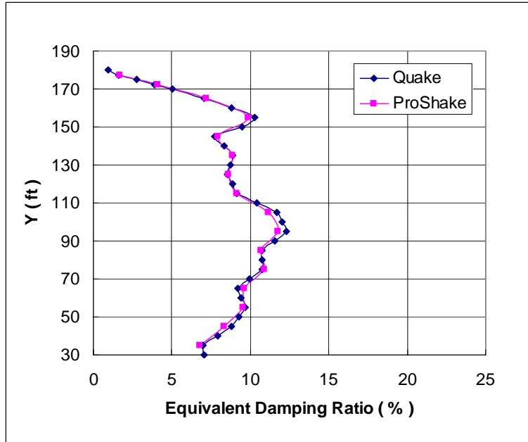
Figure 32 El Centro peak damping ratio profile
