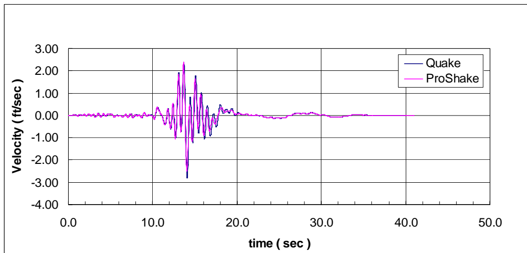
Figure 8 Treasure Island surface velocities
