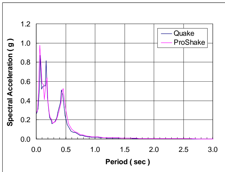
Figure 39 Saguenay spectral ground surface accelerations
