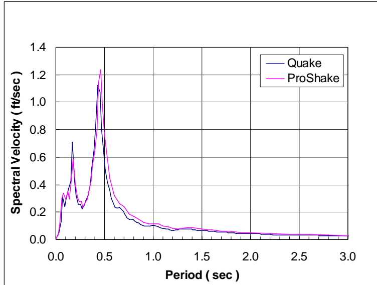
Figure 40 Saguenay spectral ground surface velocities
