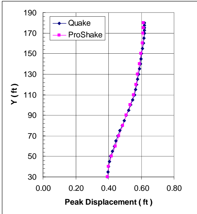
Figure 15 Treasure Island peak displacement profile
