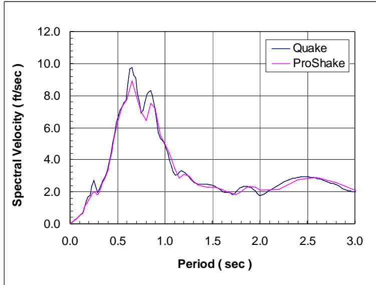
Figure 24 El Centro spectral ground surface velocity
